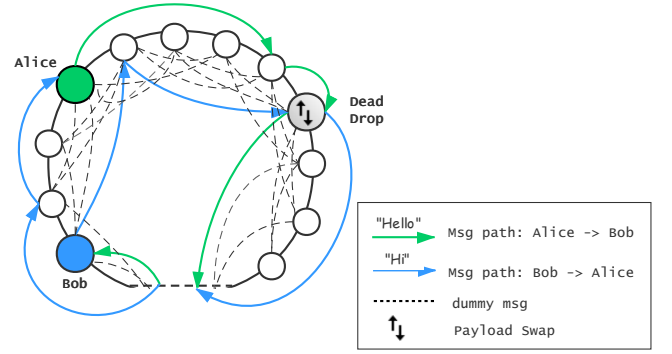
Figure 1: An example of DAENet dead drop messaging. In a communication round, Alice and Bob separately send two close-loop messages while exchanging their message payload at a randomly selected dead drop node.
