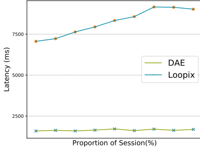
Figure 6: Latency of DAENet for anonymous communicating for varying number of sessions. The latency does not increase as the number of sessions grows.
